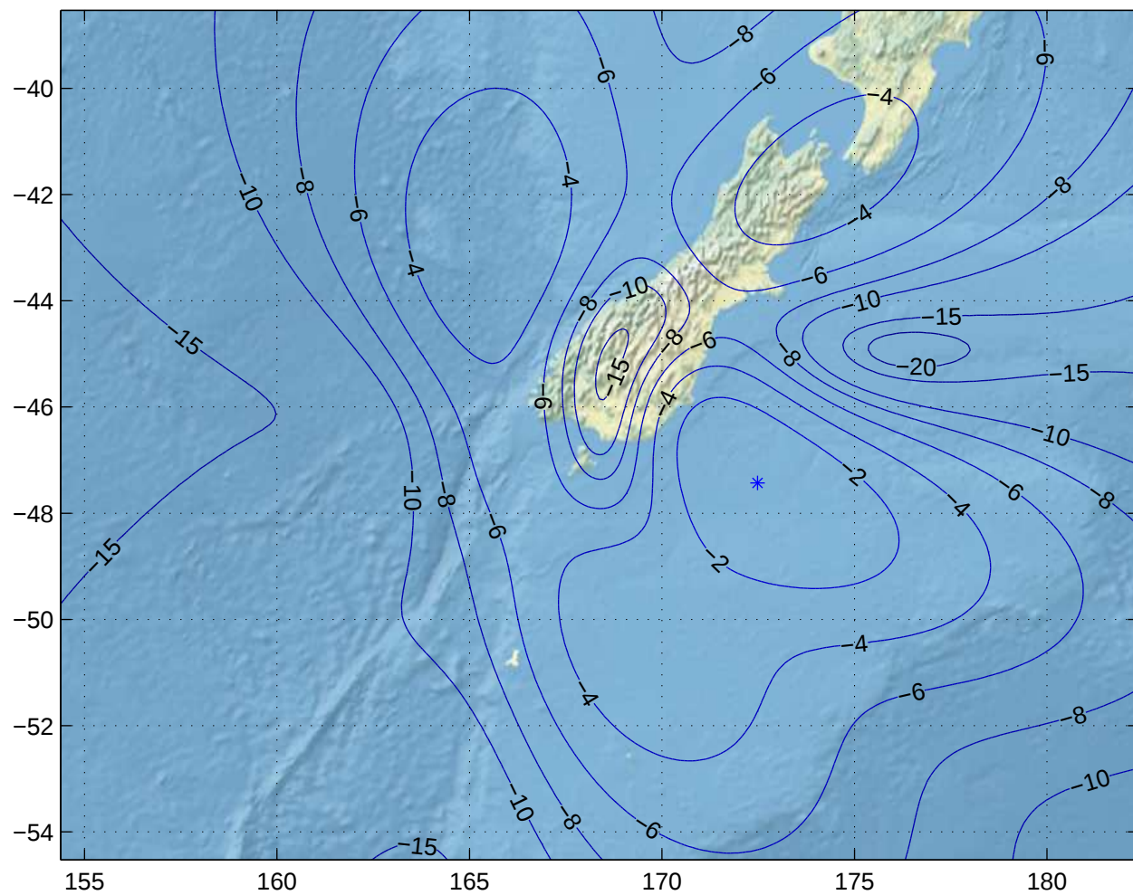
Gain Contours at 505km for IVC. Beam ID=URC, Polarization=h
