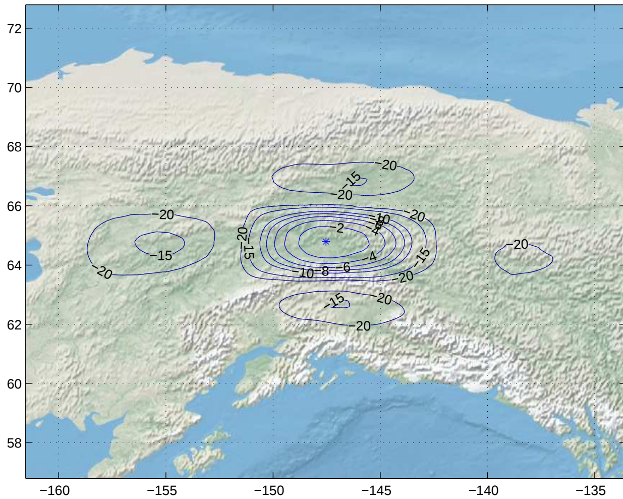
Gain Contours at 505km for FAI. Beam ID=XTC, Polarization=rhcp
