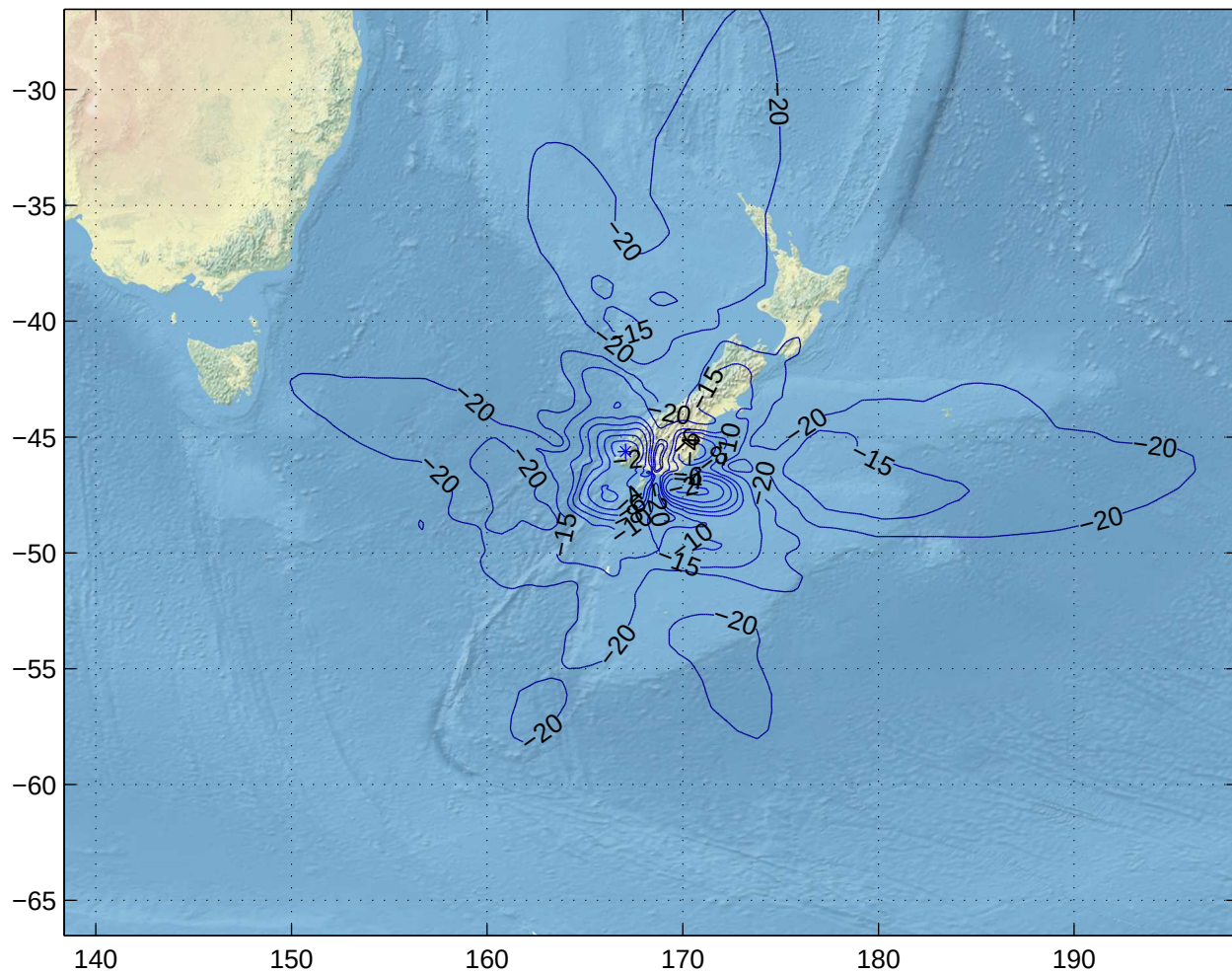
Gain Contours at 505km for IVC. Beam ID=XTX, Polarization=lhcp
