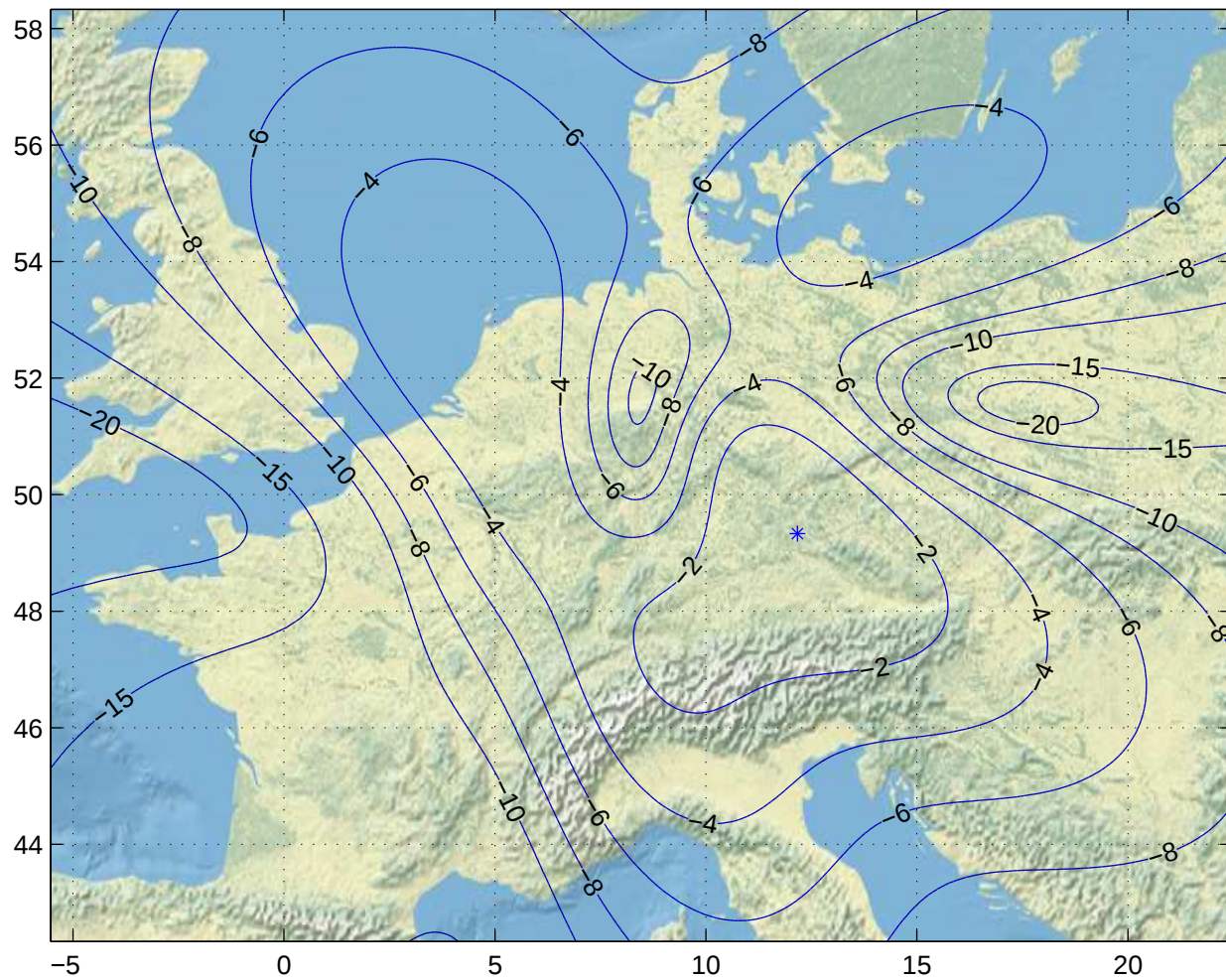
Gain Contours at 475km for FRA. Beam ID=UTC, Polarization=h
