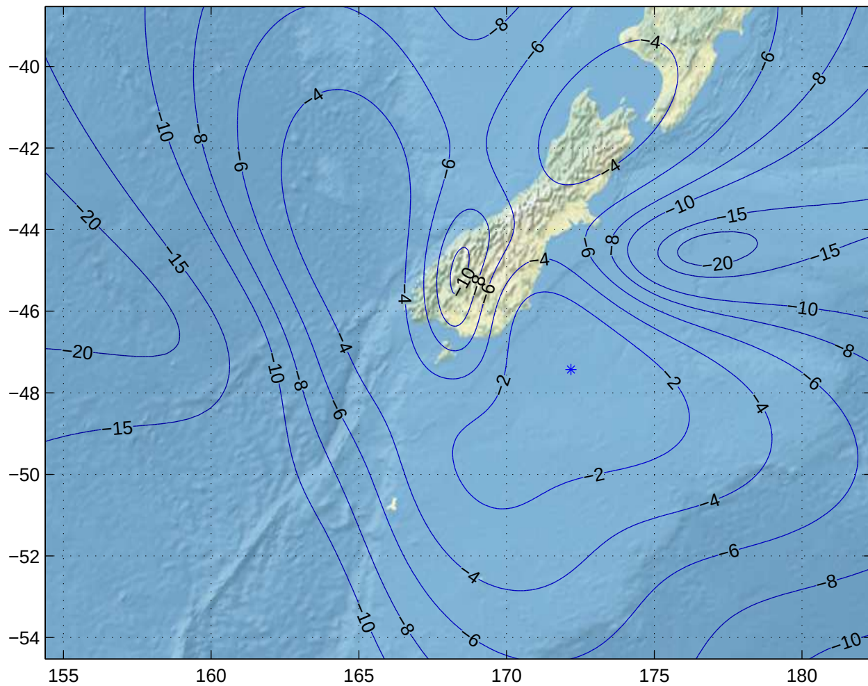
Gain Contours at 505km for IVC. Beam ID=UTC, Polarization=h
