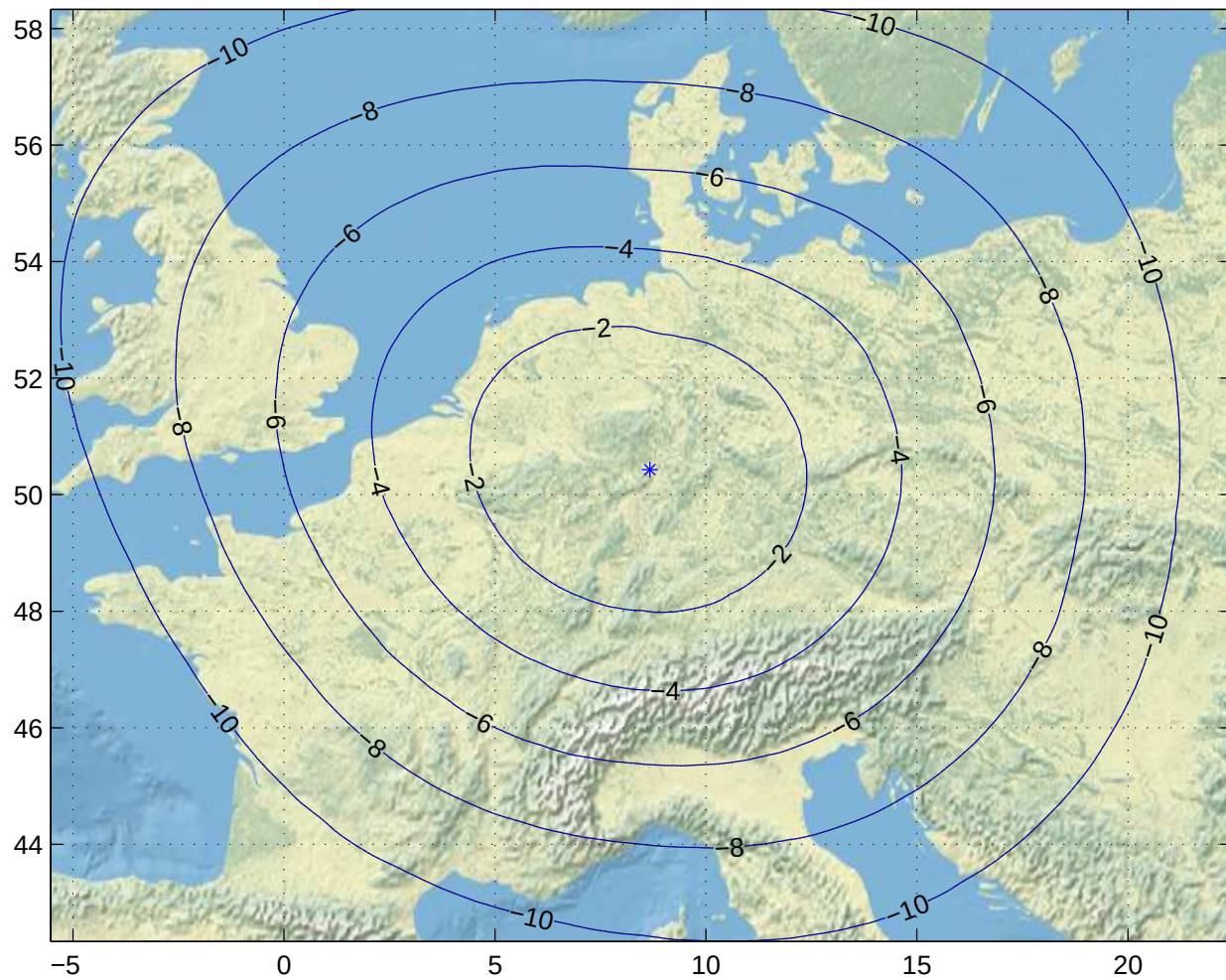
Gain Contours at 575km for FRA. Beam ID=SRC, Polarization=rhcp
