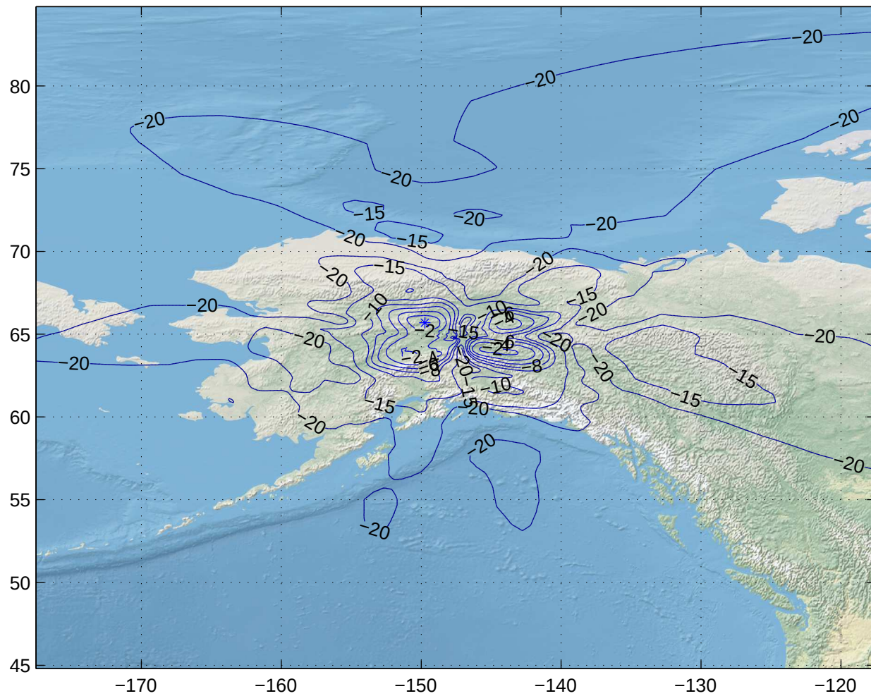
Gain Contours at 505km for FAI. Beam ID=XTX, Polarization=lhcp
