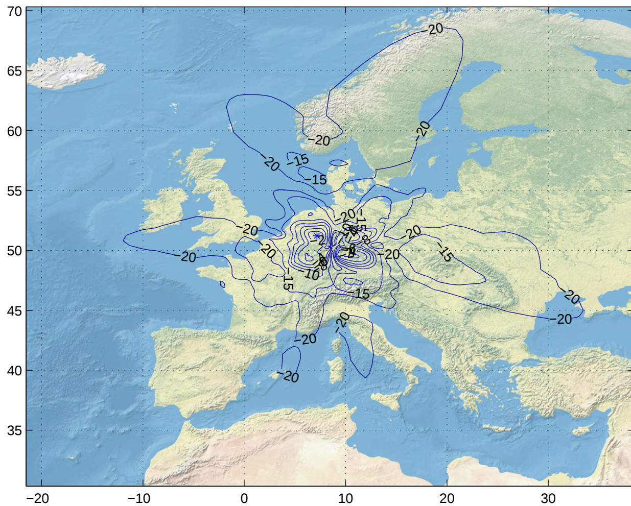
Gain Contours at 475km for FRA. Beam ID=XTX, Polarization=lhcp
