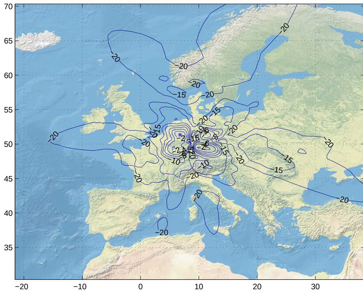
Gain Contours at 575km for FRA. Beam ID=XTX, Polarization=lhcp
