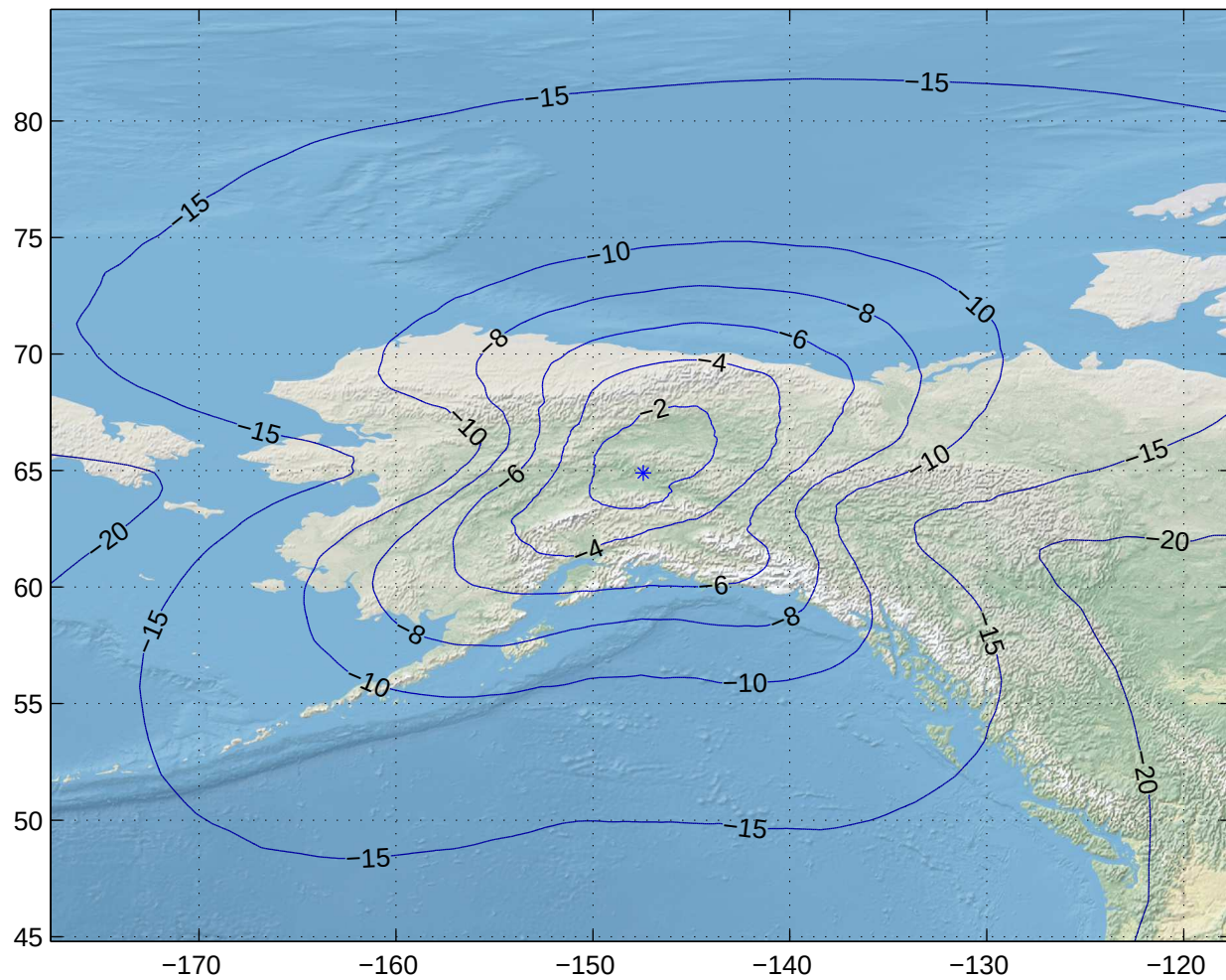
Gain Contours at 505km for FAI. Beam ID=SRX, Polarization=lhcp
