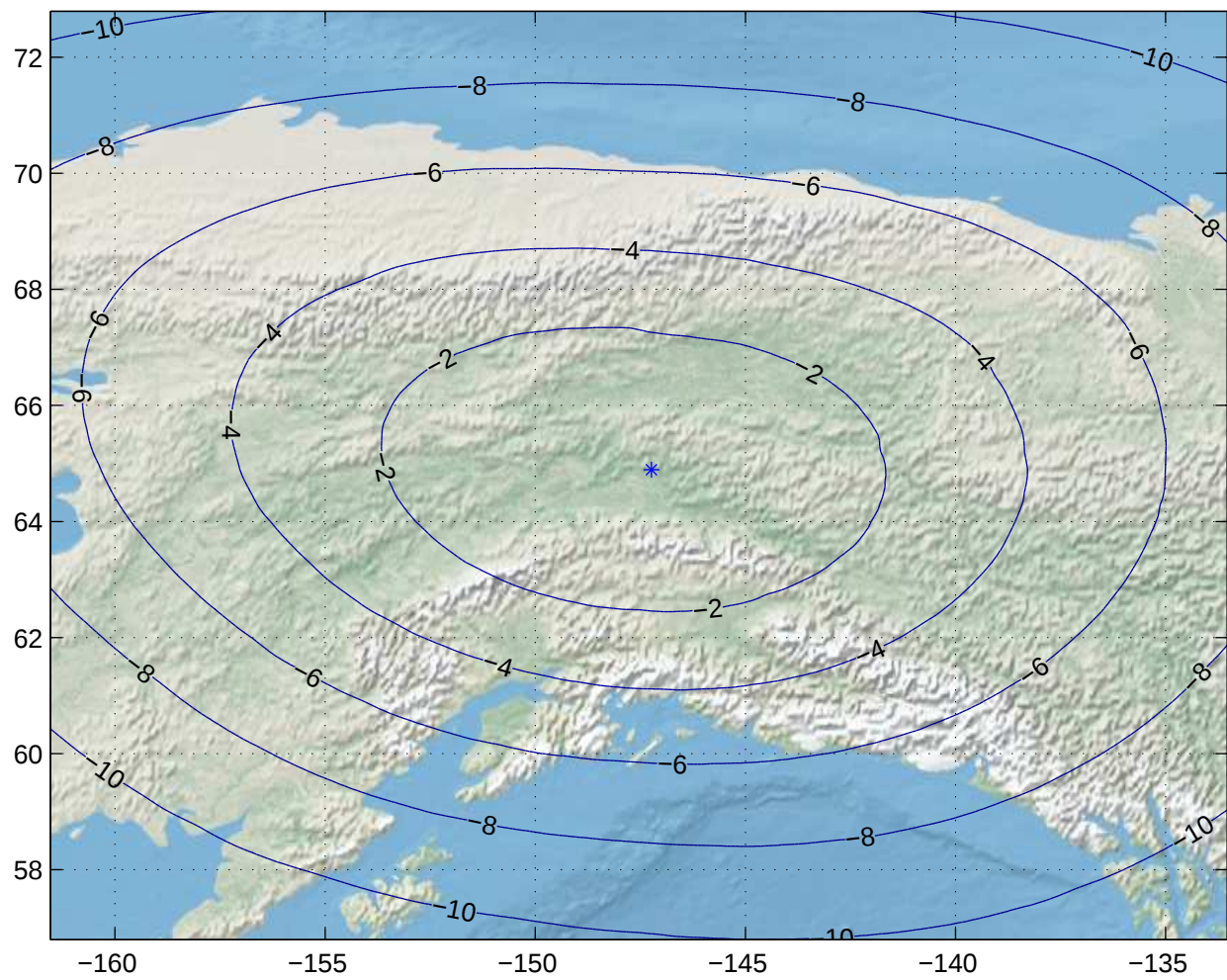
Gain Contours at 575km for FAI. Beam ID=SRC, Polarization=rhcp
