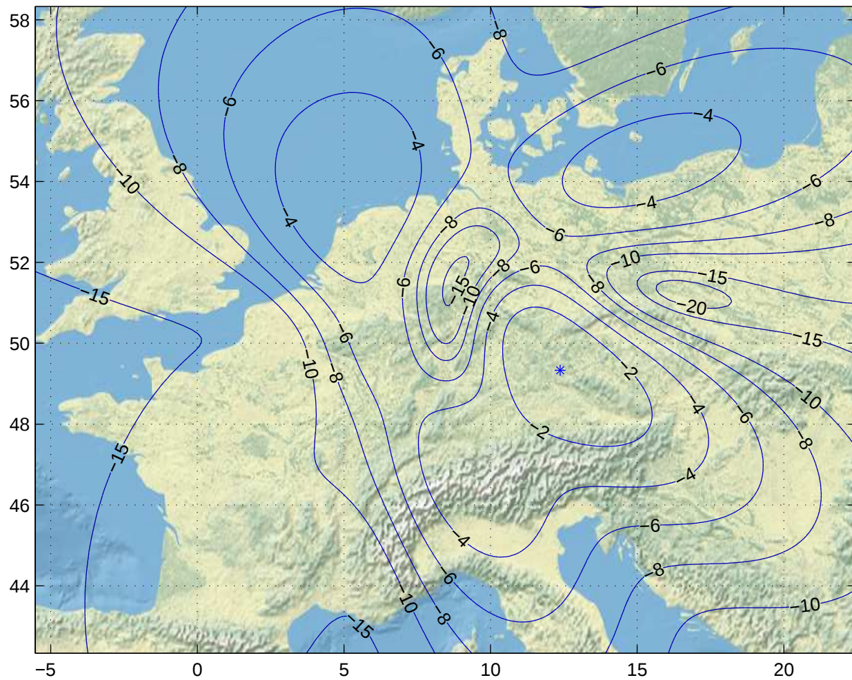
Gain Contours at 460km for FRA. Beam ID=URC, Polarization=h
