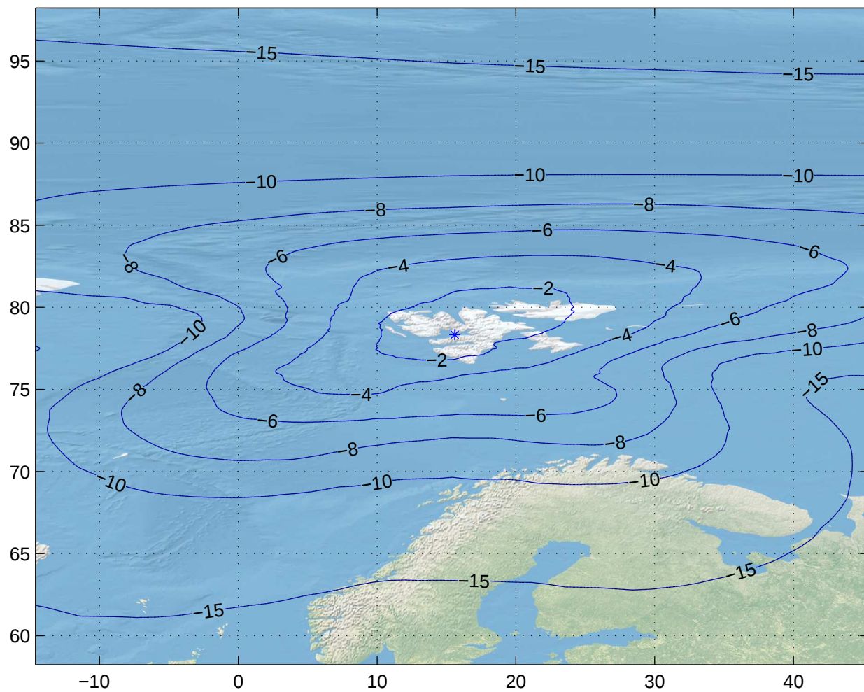
Gain Contours at 505km for LYR. Beam ID=SRX, Polarization=lhcp
