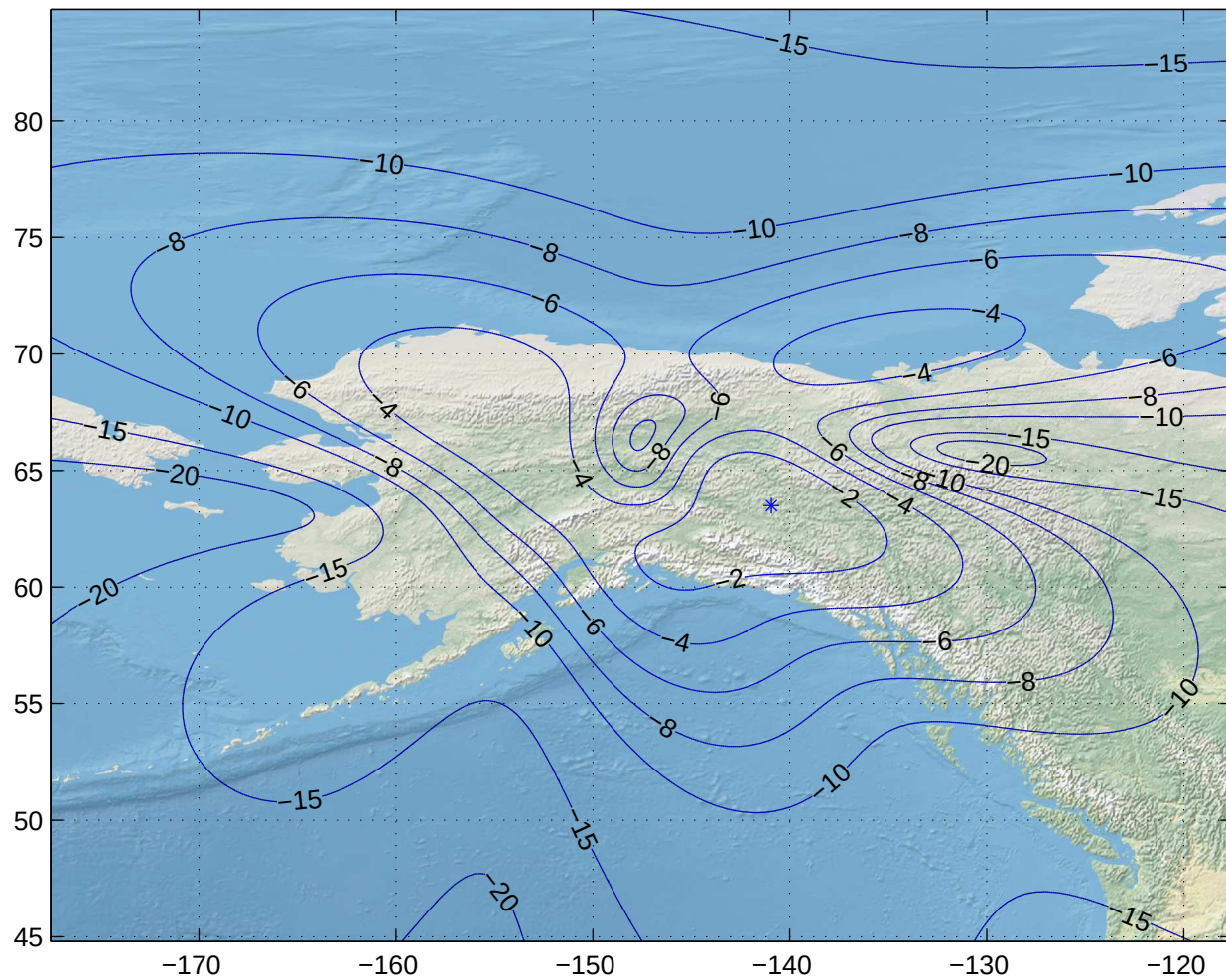
Gain Contours at 575km for FAI. Beam ID=UTX, Polarization=rhcp
