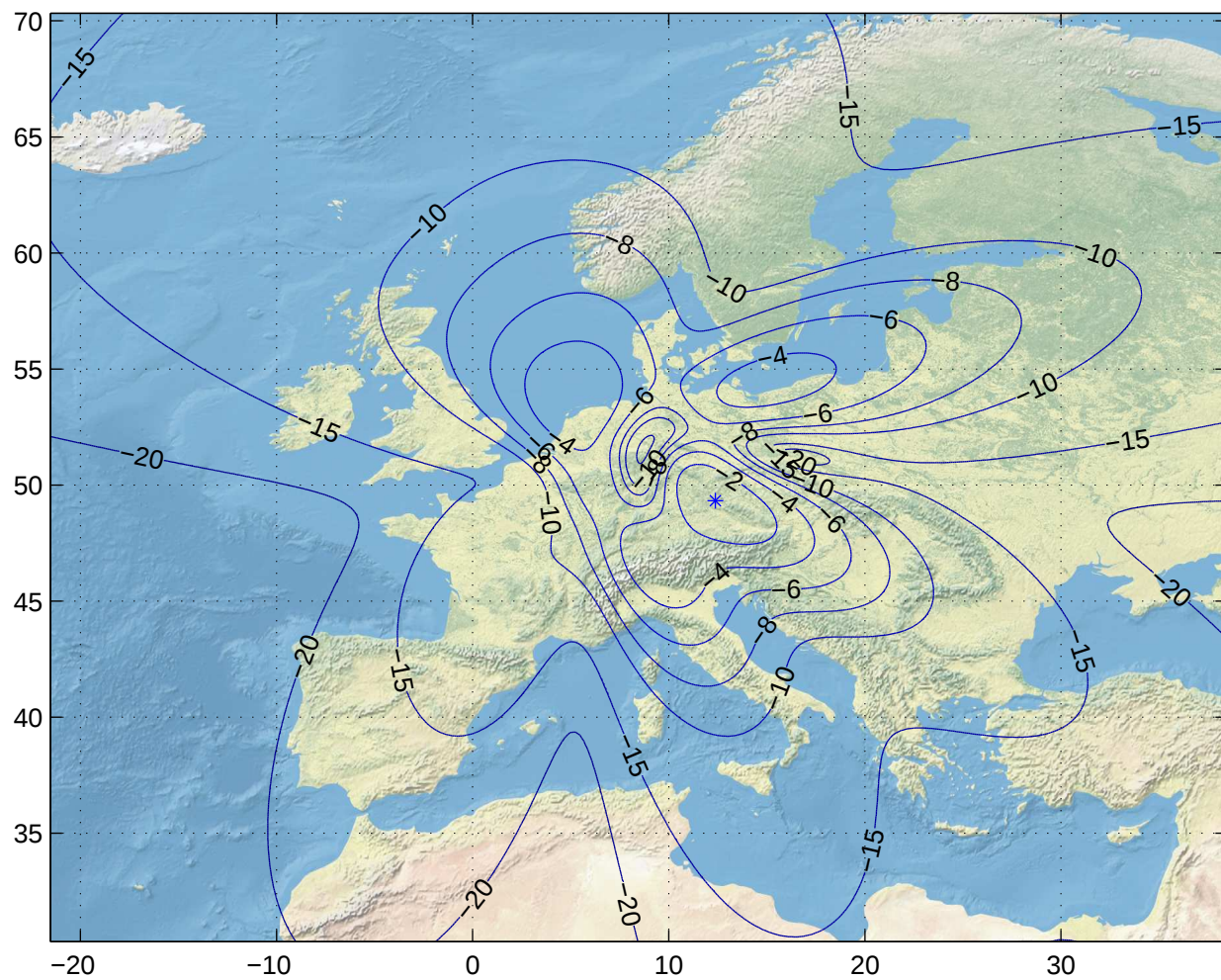
Gain Contours at 460km for FRA. Beam ID=URX, Polarization=rhcp
