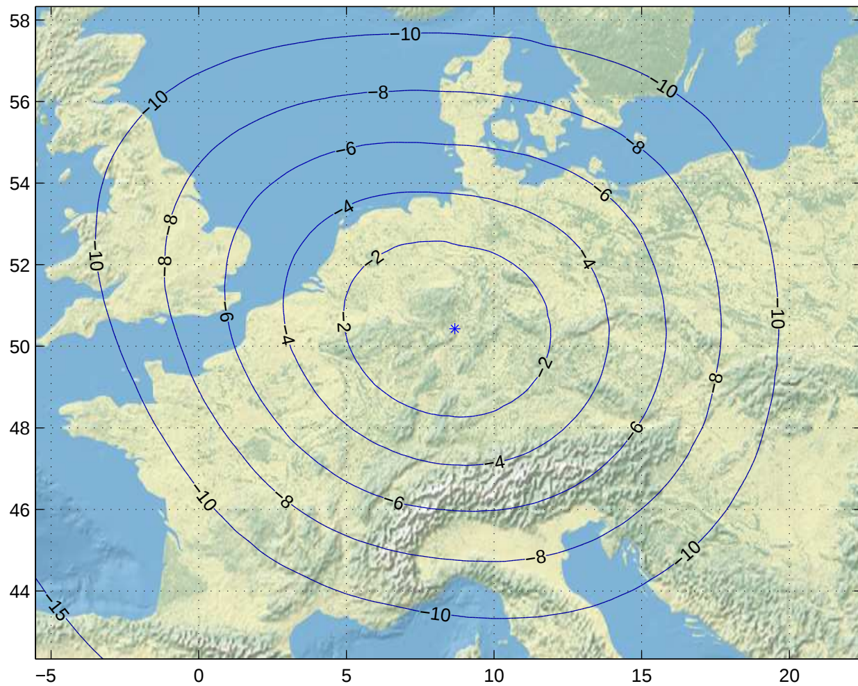
Gain Contours at 505km for FRA. Beam ID=SRC, Polarization=rhcp
