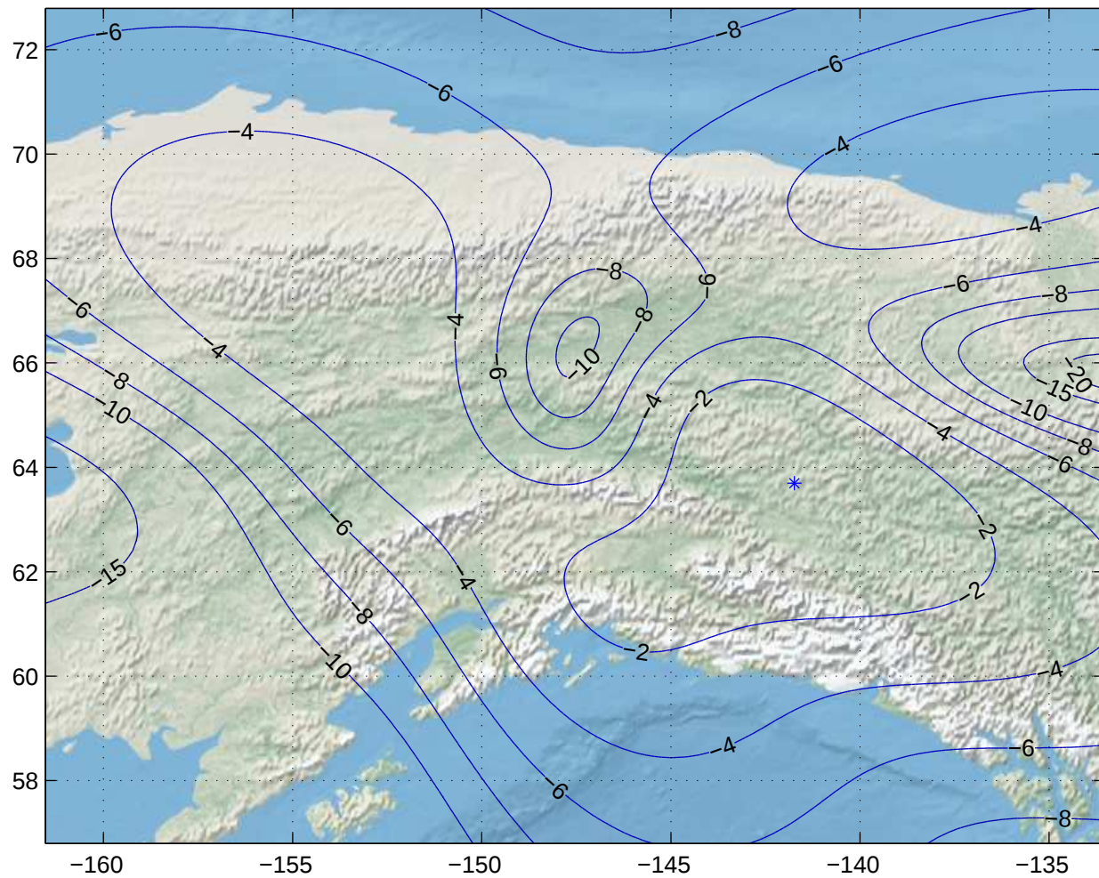
Gain Contours at 505km for FAI. Beam ID=UTC, Polarization=h
