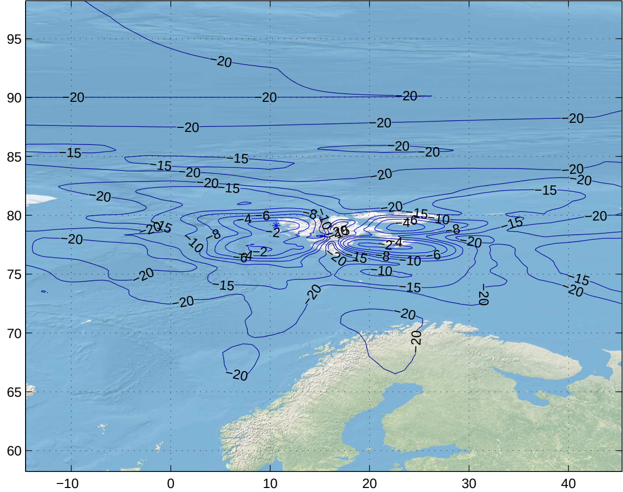
Gain Contours at 505km for LYR. Beam ID=XTX, Polarization=lhcp
