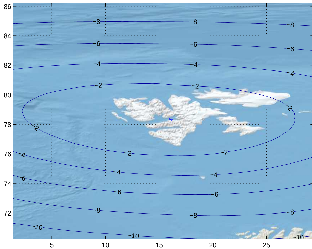
Gain Contours at 575km for LYR. Beam ID=SRC, Polarization=rhcp
