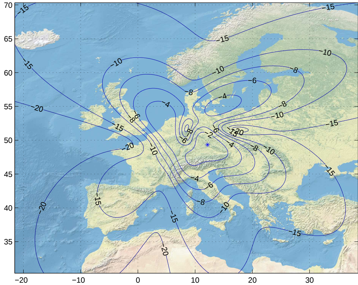
Gain Contours at 475km for FRA. Beam ID=UTX, Polarization=rhcp
