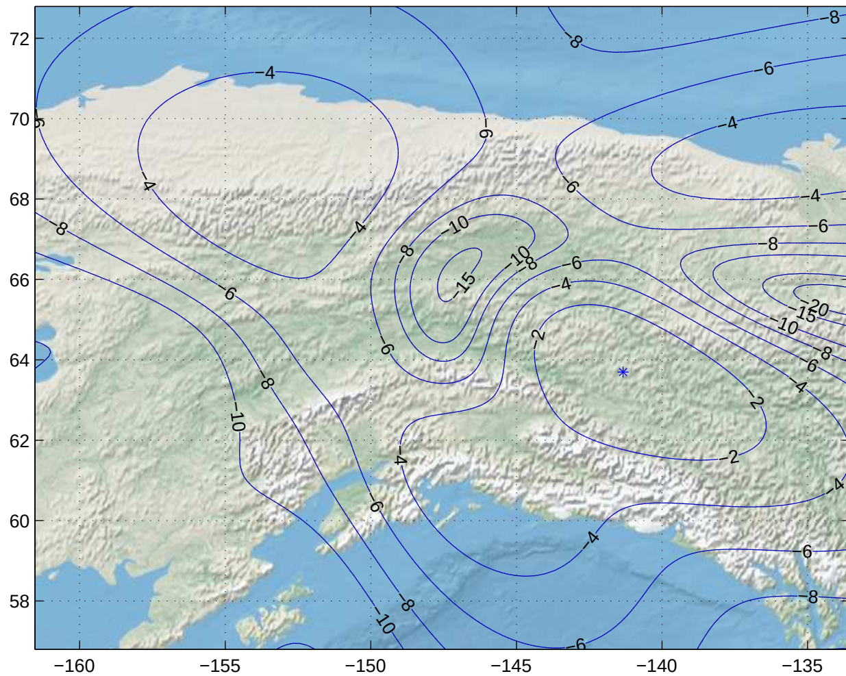
Gain Contours at 505km for FAI. Beam ID=URC, Polarization=h
