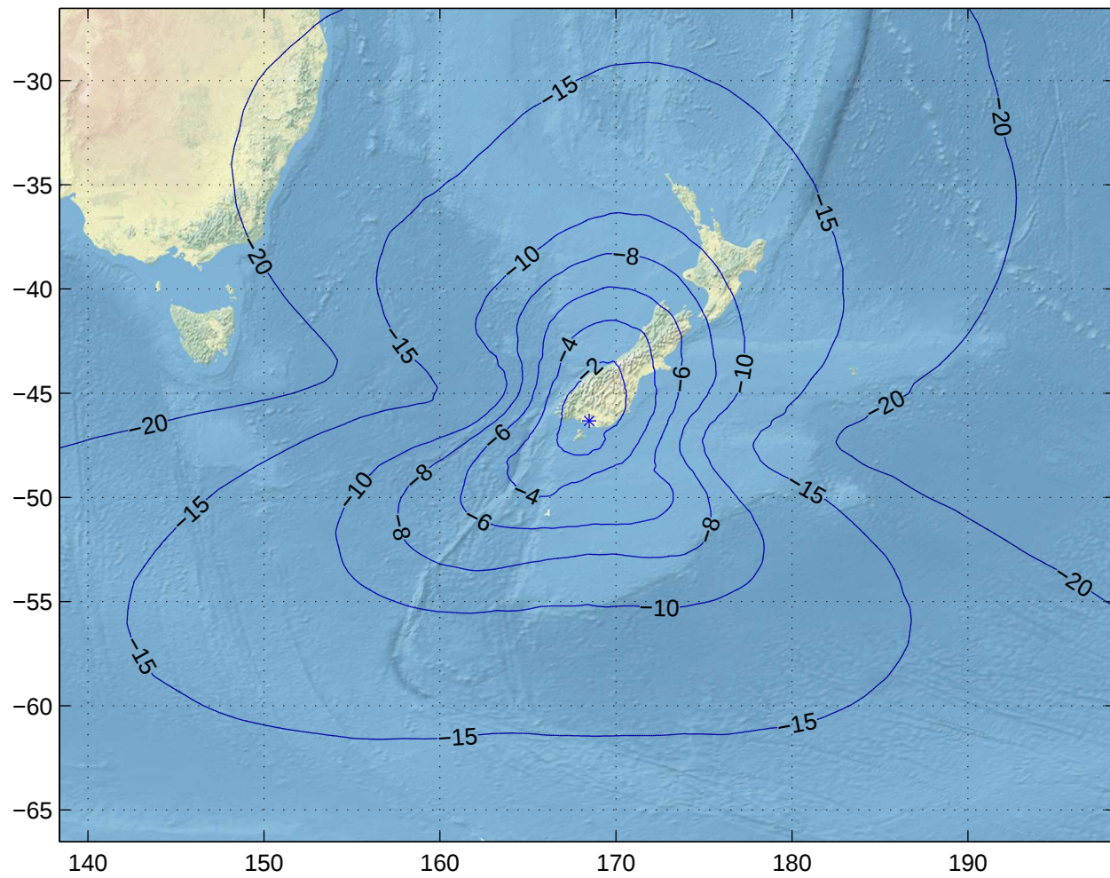
Gain Contours at 505km for IVC. Beam ID=SRX, Polarization=lhcp
