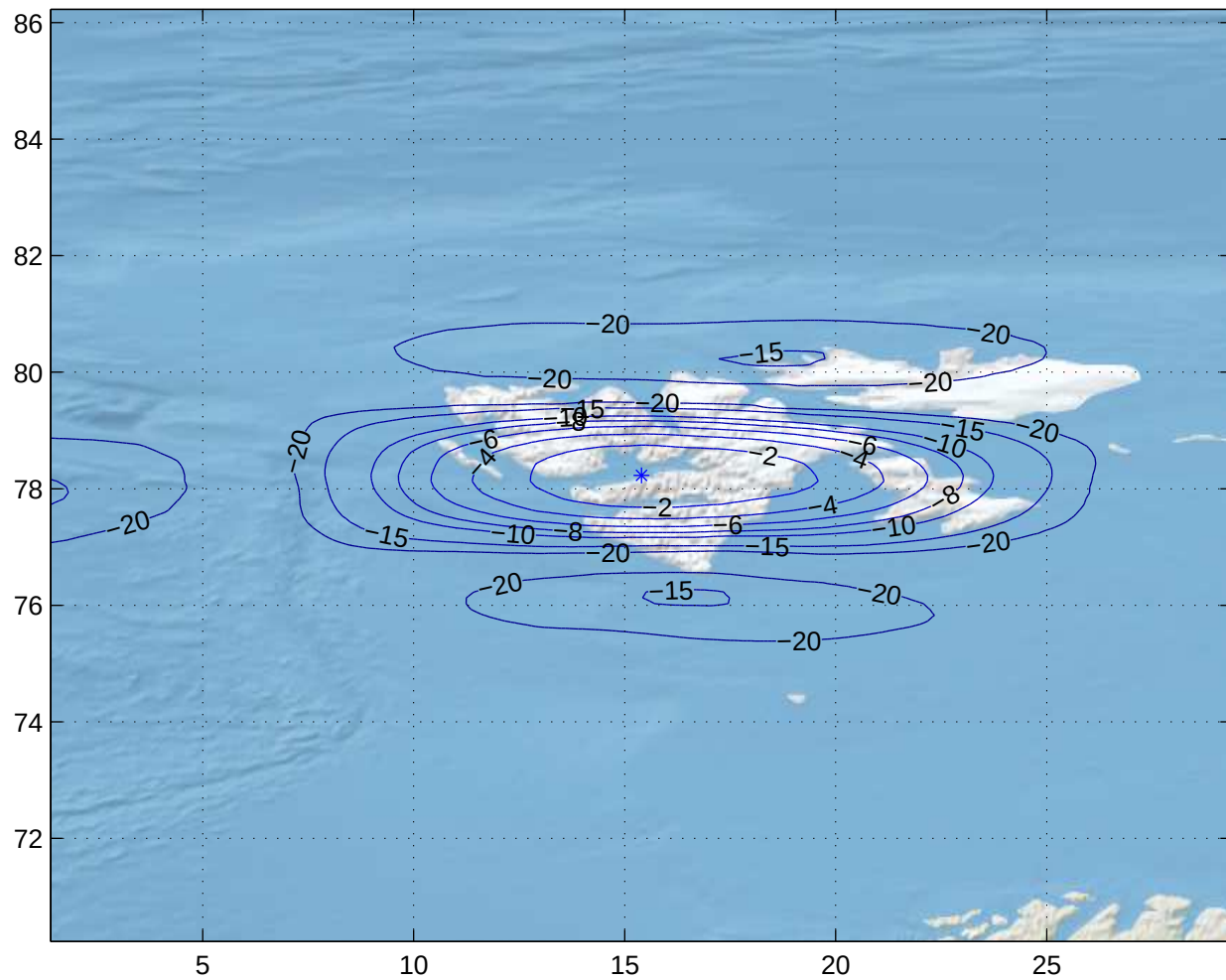
Gain Contours at 505km for LYR. Beam ID=XTC, Polarization=rhcp
