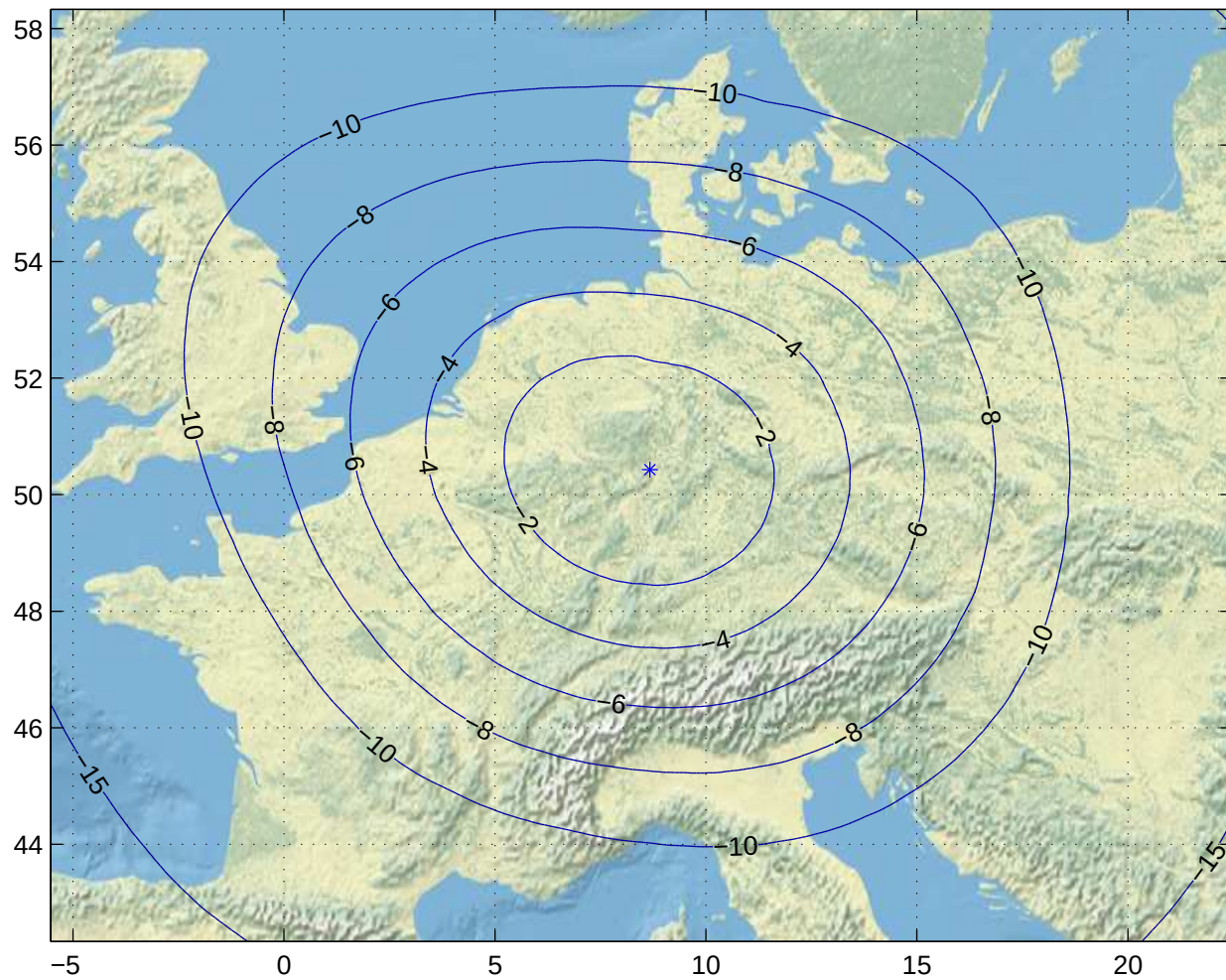
Gain Contours at 460km for FRA. Beam ID=SRC, Polarization=rhcp
