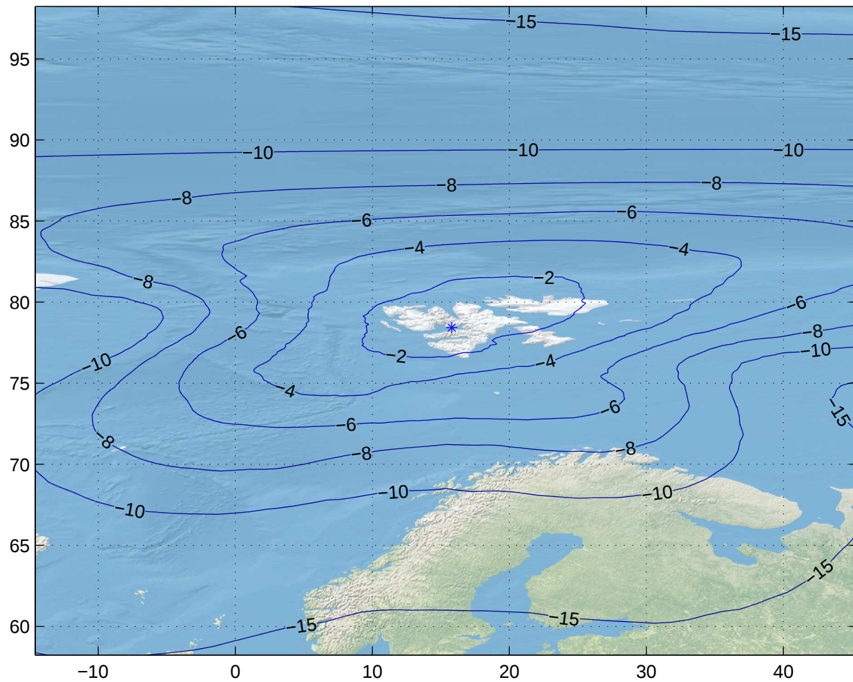
Gain Contours at 575km for LVR. Beam ID=SRX, Polarization=lhcp
