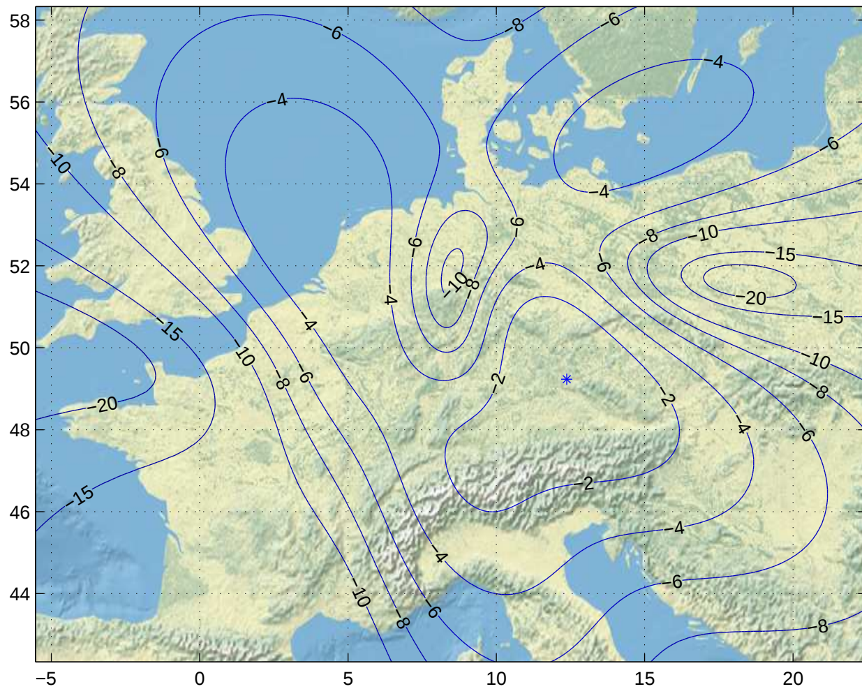
Gain Contours at 505km for FRA. Beam ID=UTC, Polarization=h
