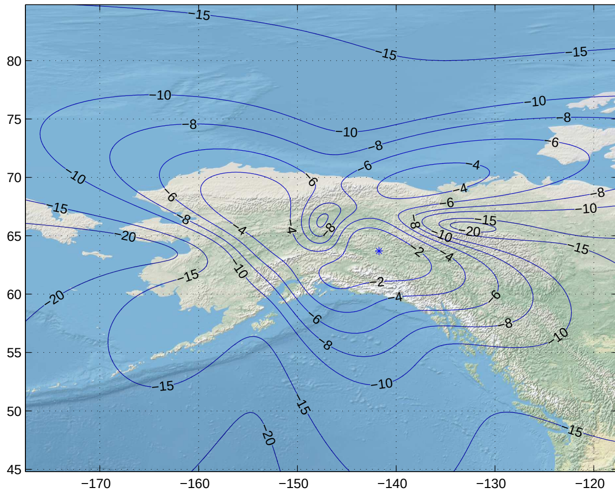
Gain Contours at 505km for FAI. Beam ID=UTX, Polarization=rhcp
