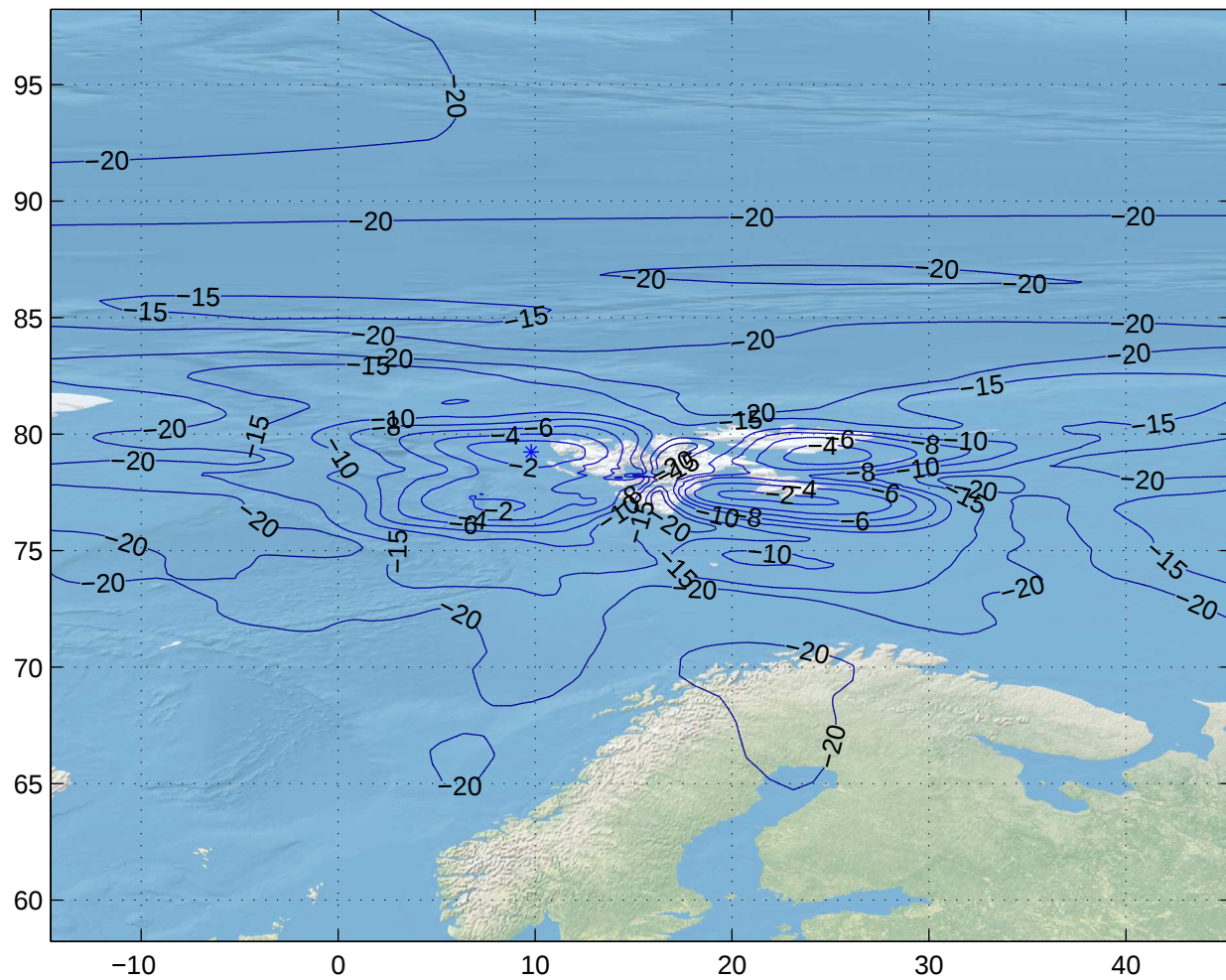
Gain Contours at 575km for LYR. Beam ID=XTX, Polarization=lhcp
