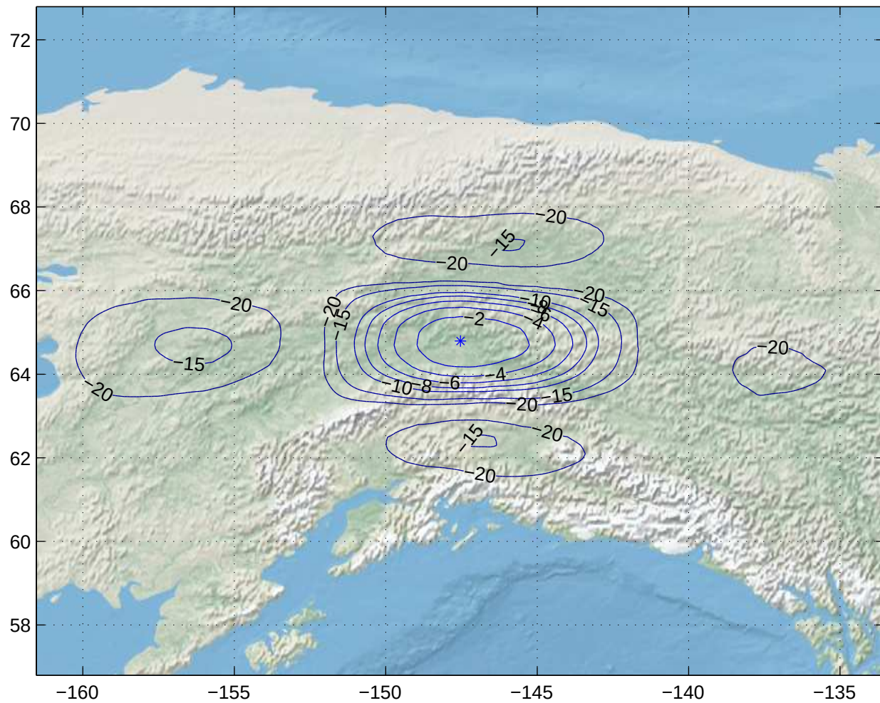
Gain Contours at 575km for FAI. Beam ID=XTC, Polarization=rhcp
