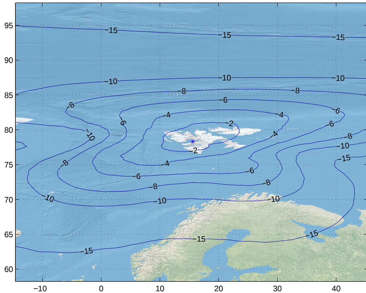
Gain Contours at 475km for LYR. Beam ID=SRX, Polarization=lhcp
