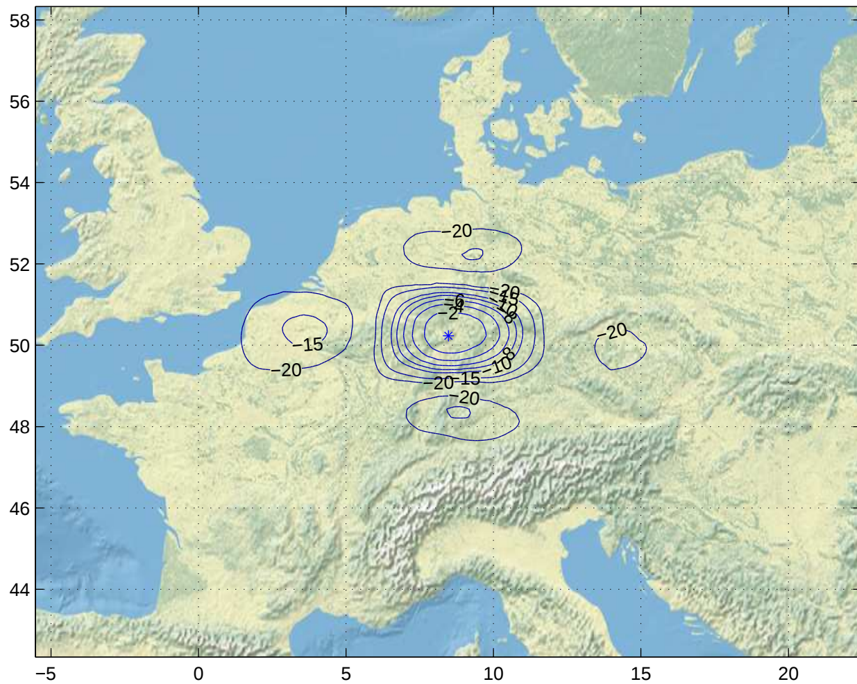
Gain Contours at 475km for FRA. Beam ID=XTC, Polarization=rhcp
