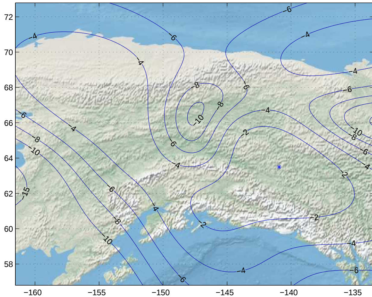
Gain Contours at 575km for FAI. Beam ID=UTC, Polarization=h
