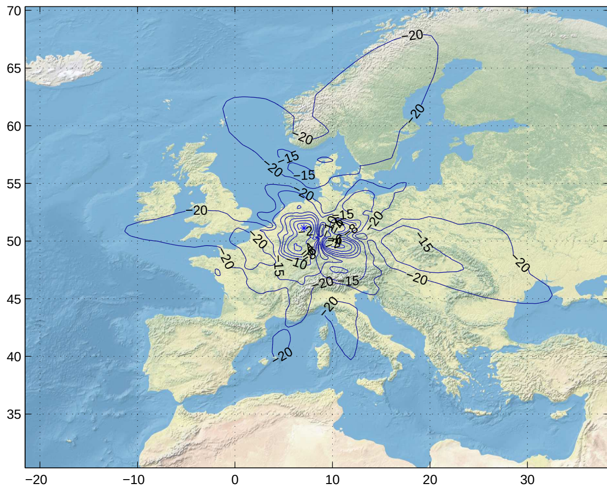
Gain Contours at 460km for FRA. Beam ID=XTX, Polarization=lhcp
