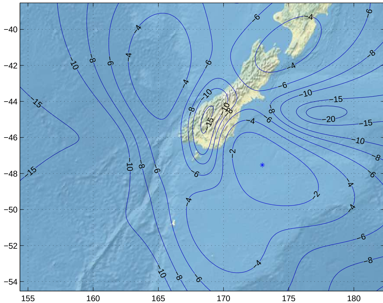
Gain Contours at 575km for IVC. Beam ID=URC, Polarization=h
