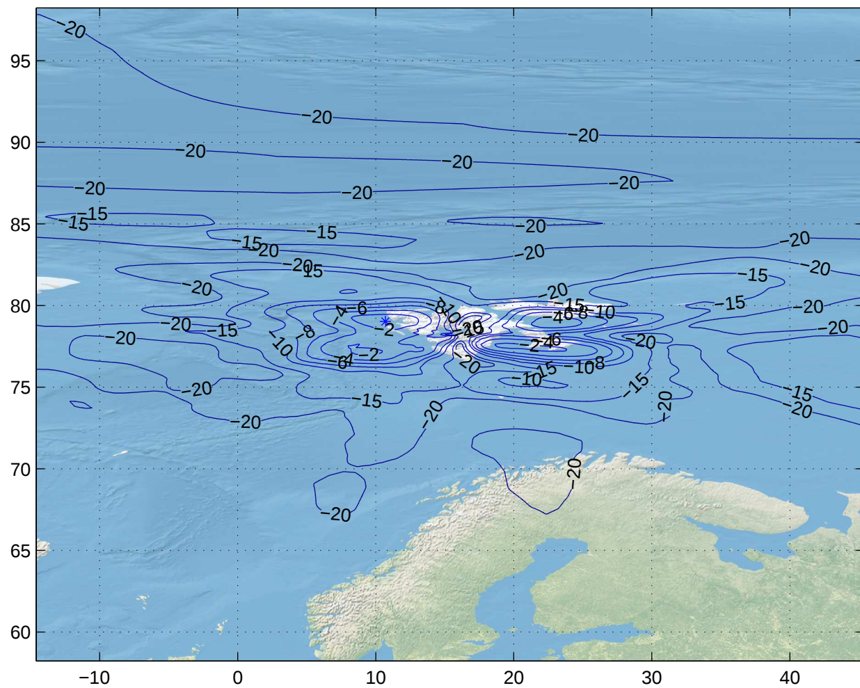
Gain Contours at 475km for LYR. Beam ID=XTX, Polarization=lhcp
