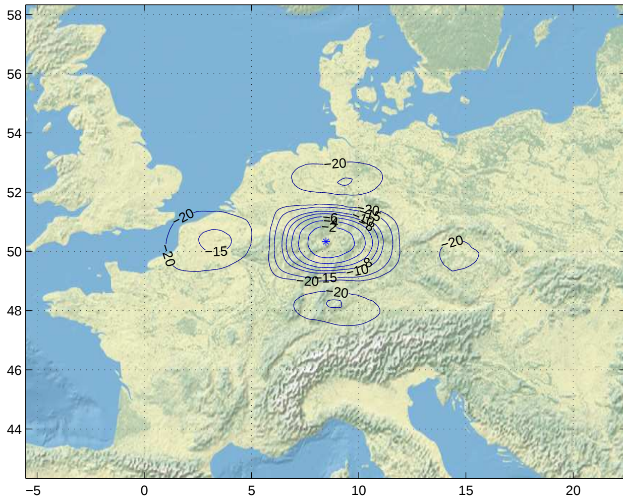
Gain Contours at 505km for FRA. Beam ID=XTC, Polarization=rhcp
