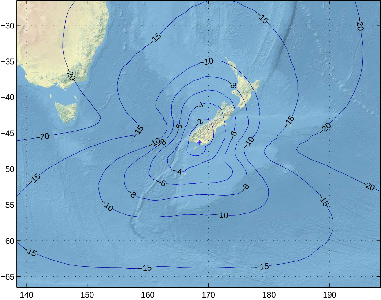
Gain Contours at 575km for IVC. Beam ID=SRX, Polarization=lhcp
