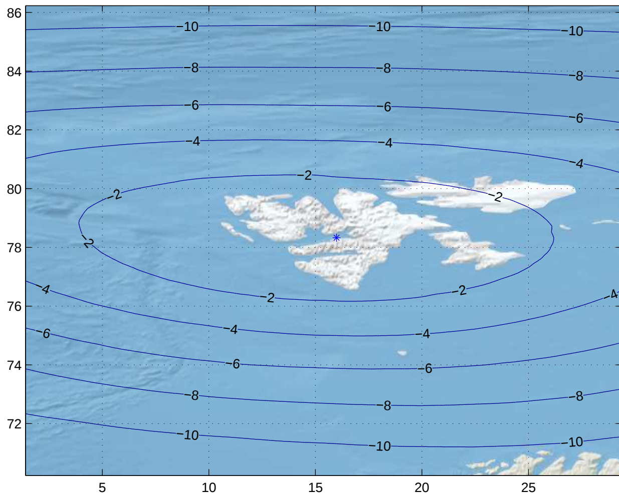
Gain Contours at 505km for LYR. Beam ID=SRC, Polarization=rhcp
