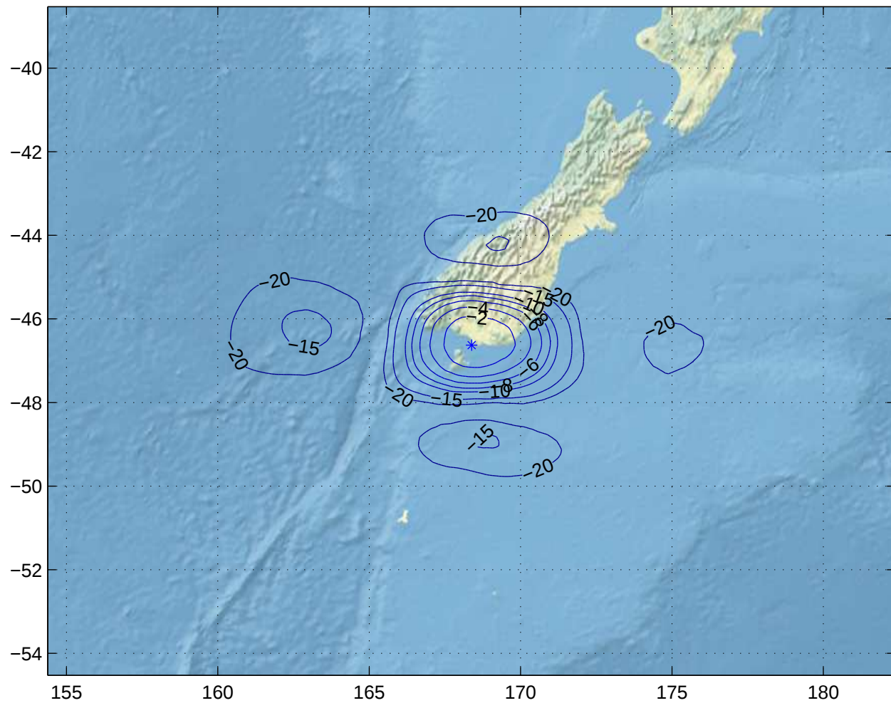
Gain Contours at 575km for IVC. Beam ID=XTC, Polarization=rhcp
