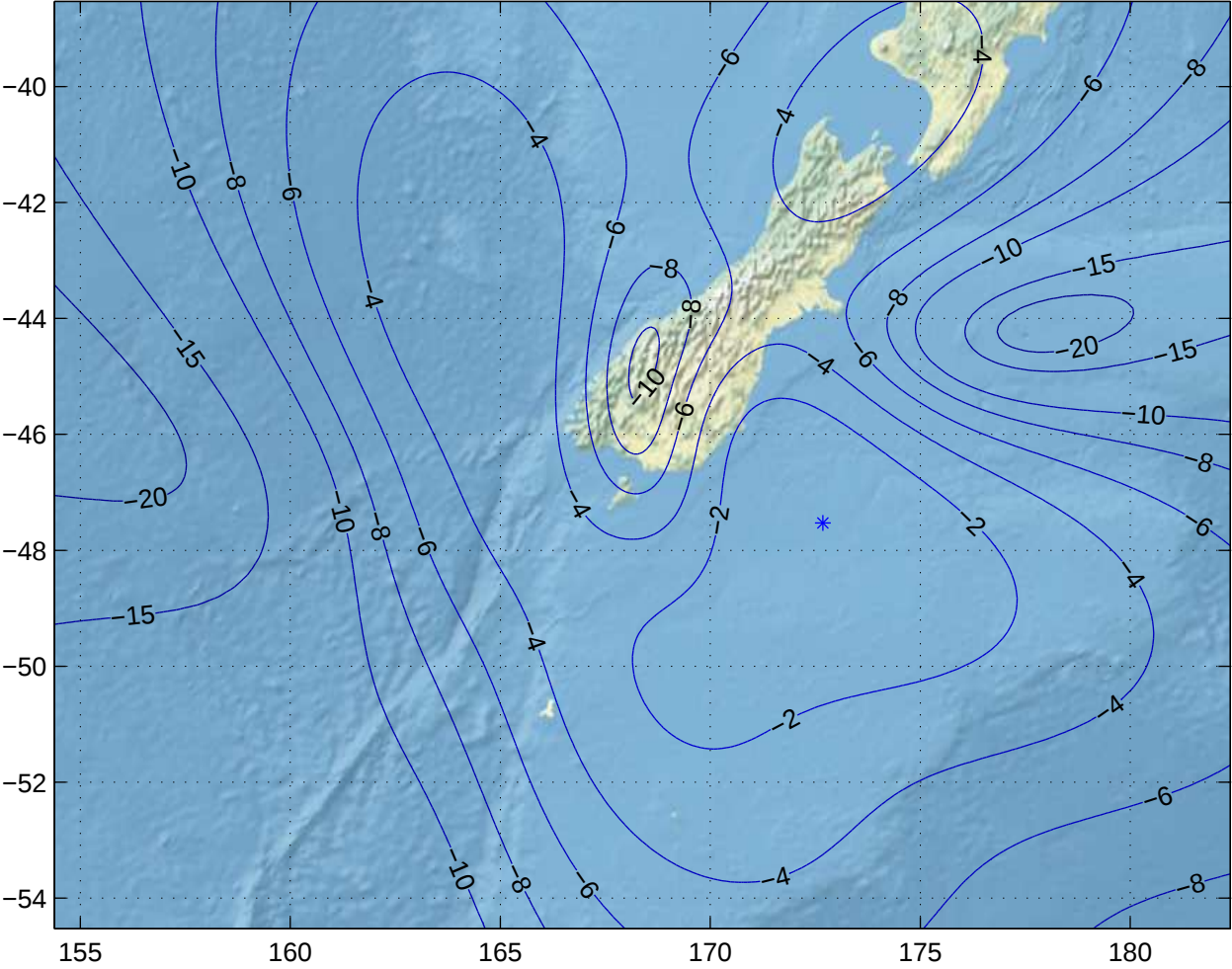
Gain Contours at 575km for IVC. Beam ID=UTC, Polarization=h
