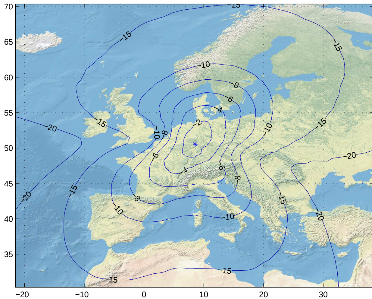
Gain Contours at 575km for FRA. Beam ID=SRX, Polarization=lhcp
