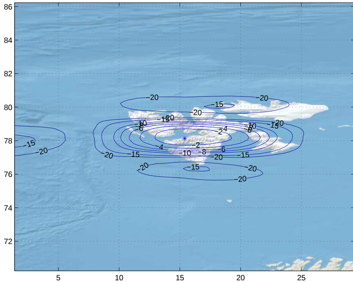
Gain Contours at 460km for LYR. Beam ID=XTC, Polarization=rhcp
