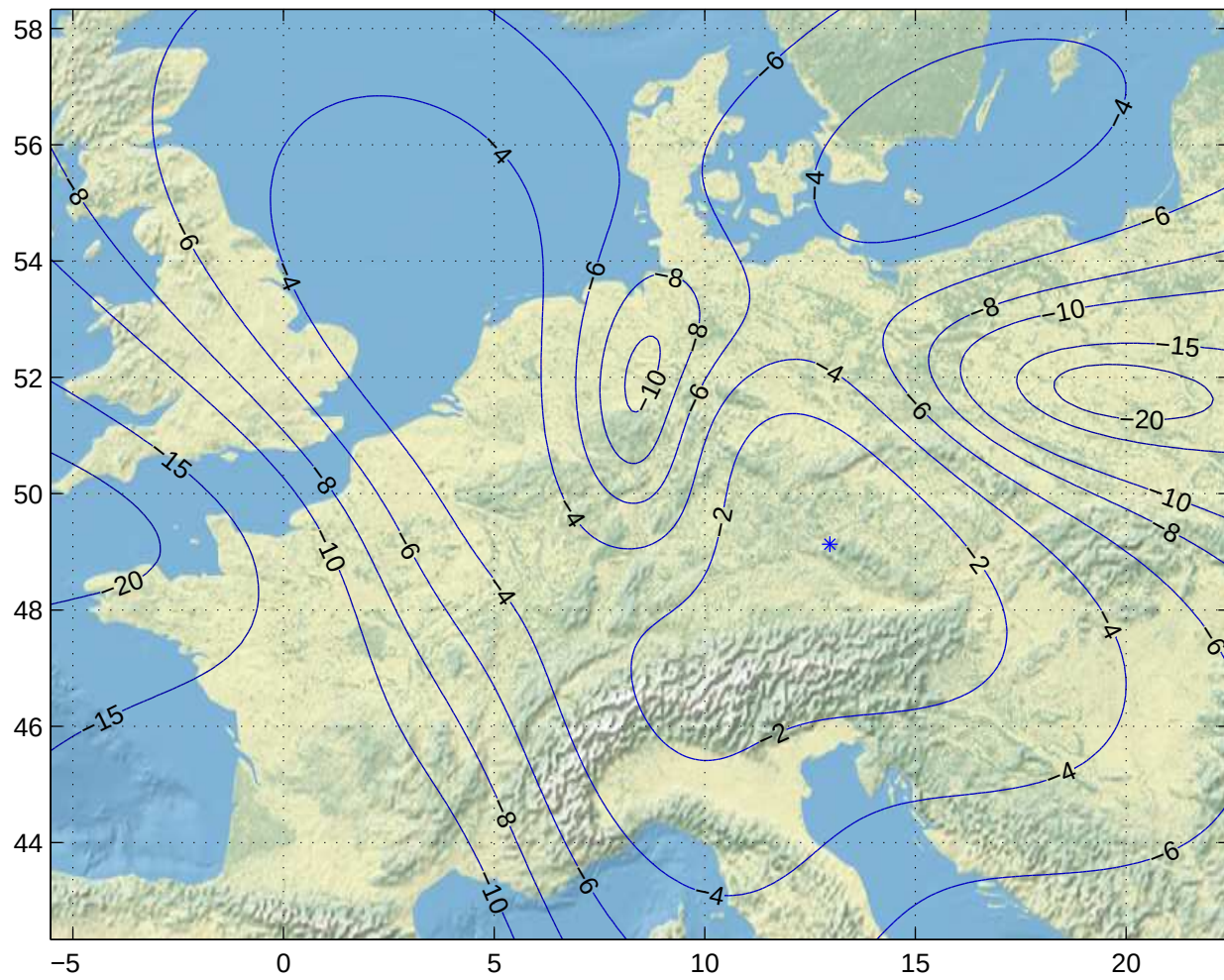
Gain Contours at 575km for FRA. Beam ID=UTC, Polarization=h
