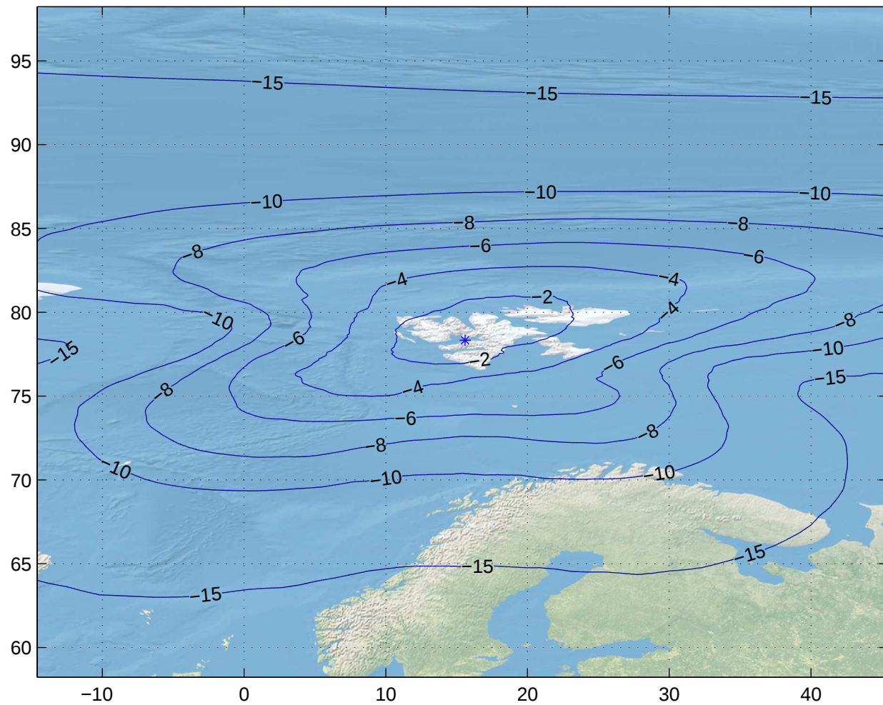
Gain Contours at 460km for LYR. Beam ID=SRX, Polarization=lhcp
