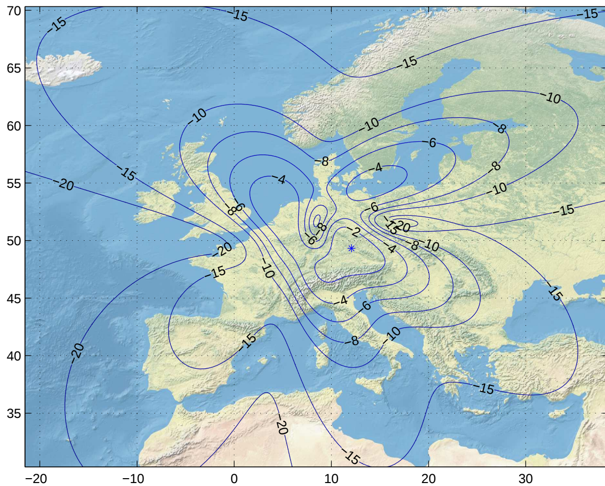
Gain Contours at 460km for FRA. Beam ID=UTX, Polarization=rhcp
