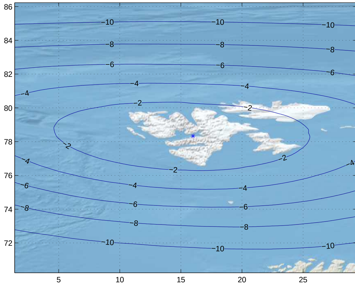
Gain Contours at 475km for LYR. Beam ID=SRC, Polarization=rhcp
