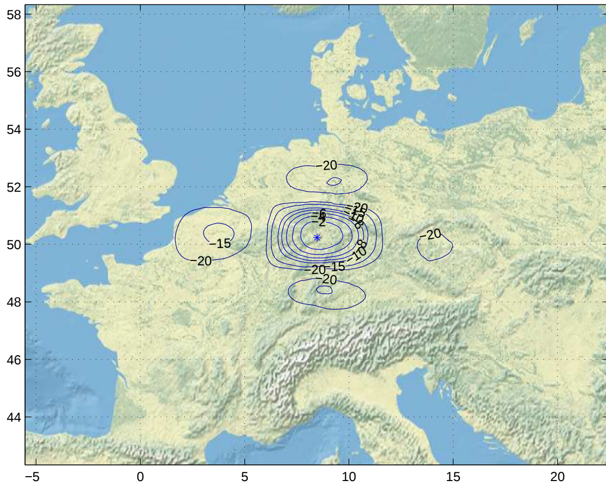
Gain Contours at 460km for FRA. Beam ID=XTC, Polarization=rhcp
