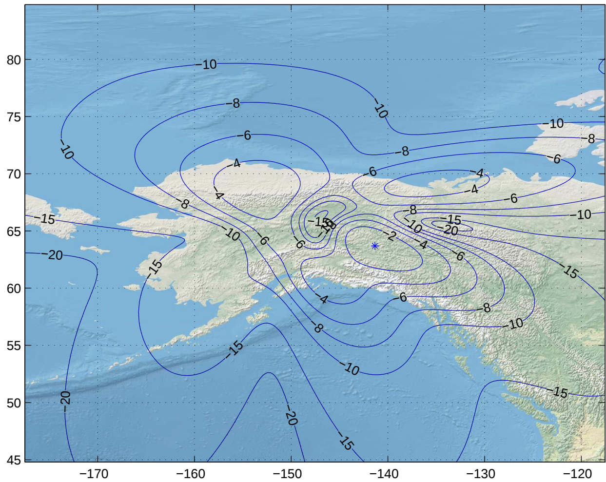
Gain Contours at 505km for FAI. Beam ID=URX, Polarization=rhcp
