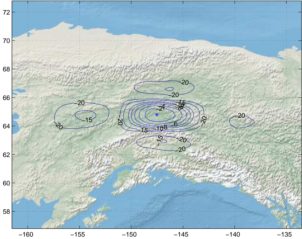
Gain Contours at 450km for FAI. Beam ID=XTC, Polarization=rhcp
