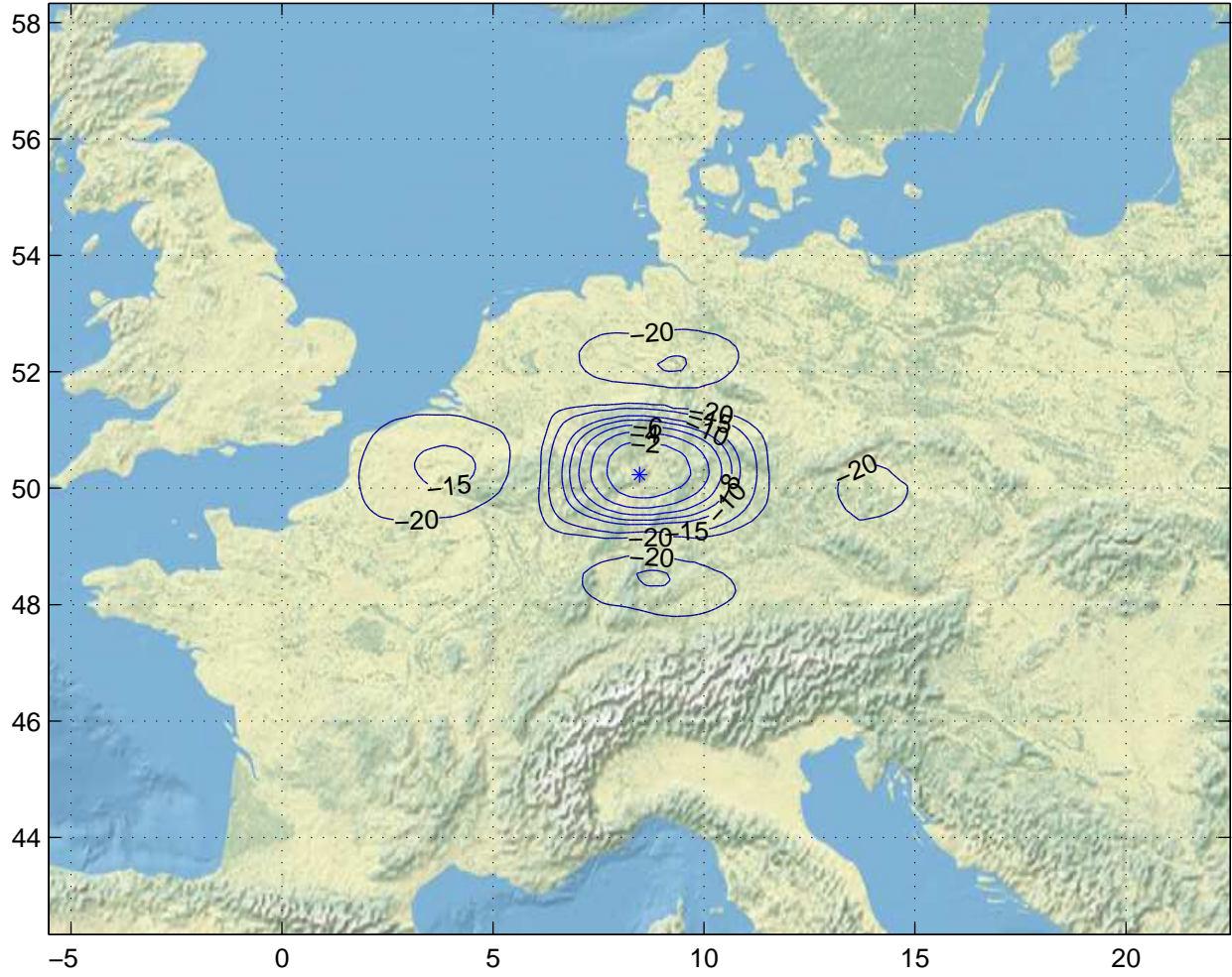
Gain Contours at 450km for FRA. Beam ID=XTC, Polarization=rhcp
